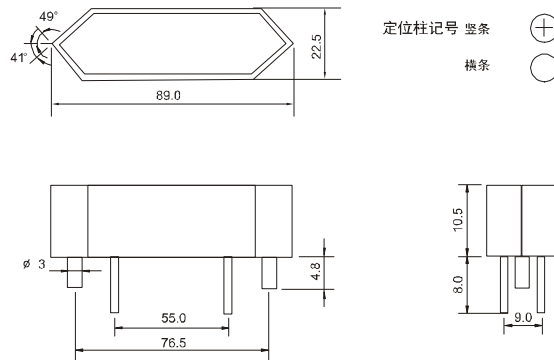
ASSEMBLY BOARD
